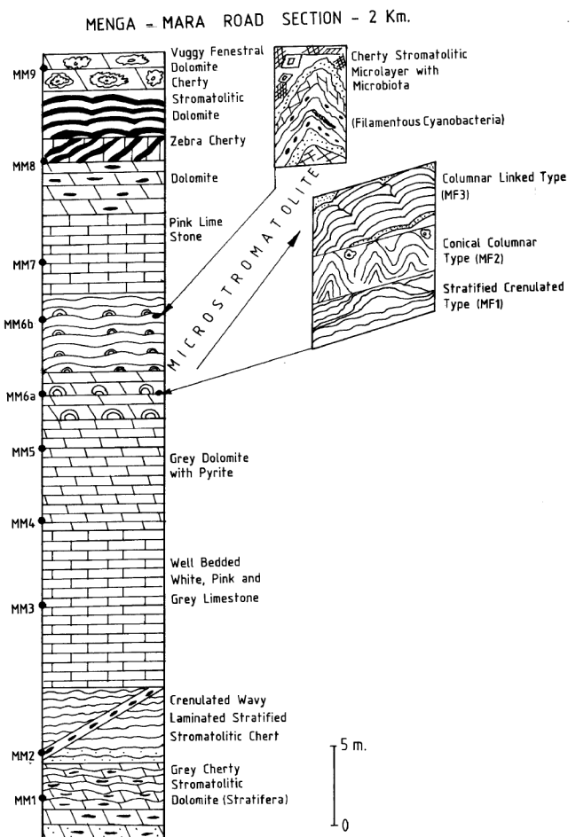
Figure 2. Litholog of microstromatolitic Menga Limestone, Menga-Mara road section, 2 km from Menga village.
