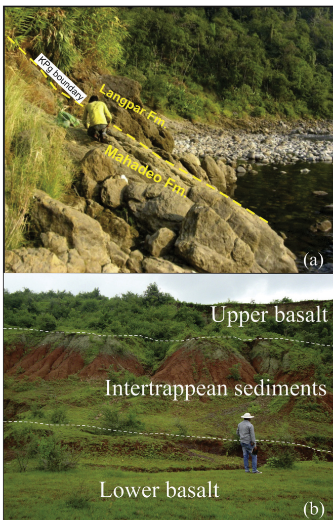
Fig. 5. Field aspects of the two sampled sections in India: (A) KPg boundary location between the Mahadeo and Langpar formations in an Um Sohrynkew River section, not far from Theria village, Shillong Plateau, northeastern India; (B) Jhilmili section showing the two basalt traps and sandwiched intertrappean sedimentary rocks.
