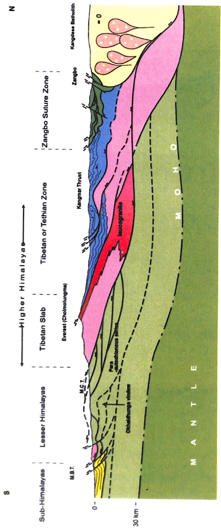
Figure 4: Sketch section of the Everest traverse.
