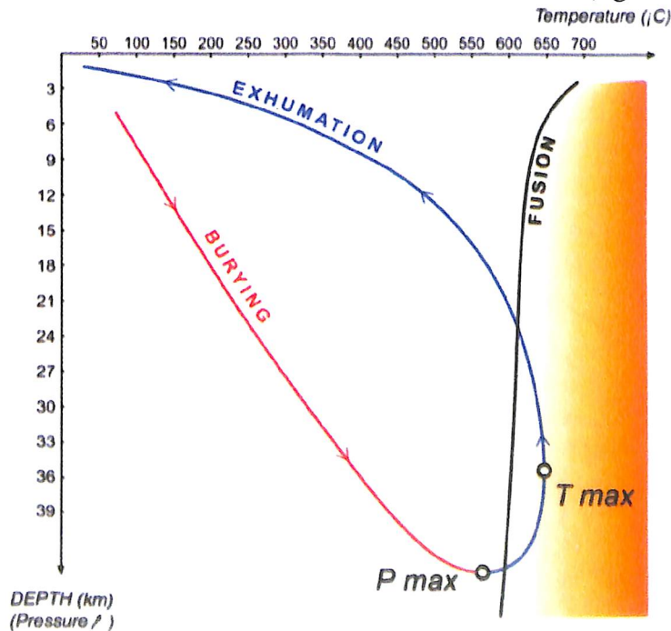
Figure.5: Models of burying and exhumation .
