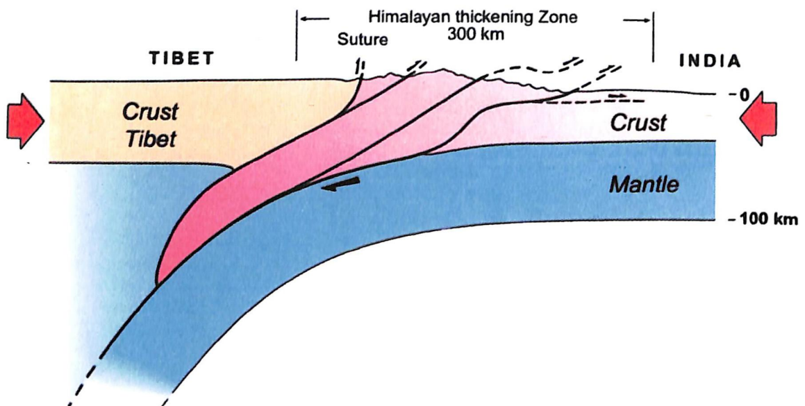
Figure. 2: Sketch section of the Himalayan accretionary thickened zone.
