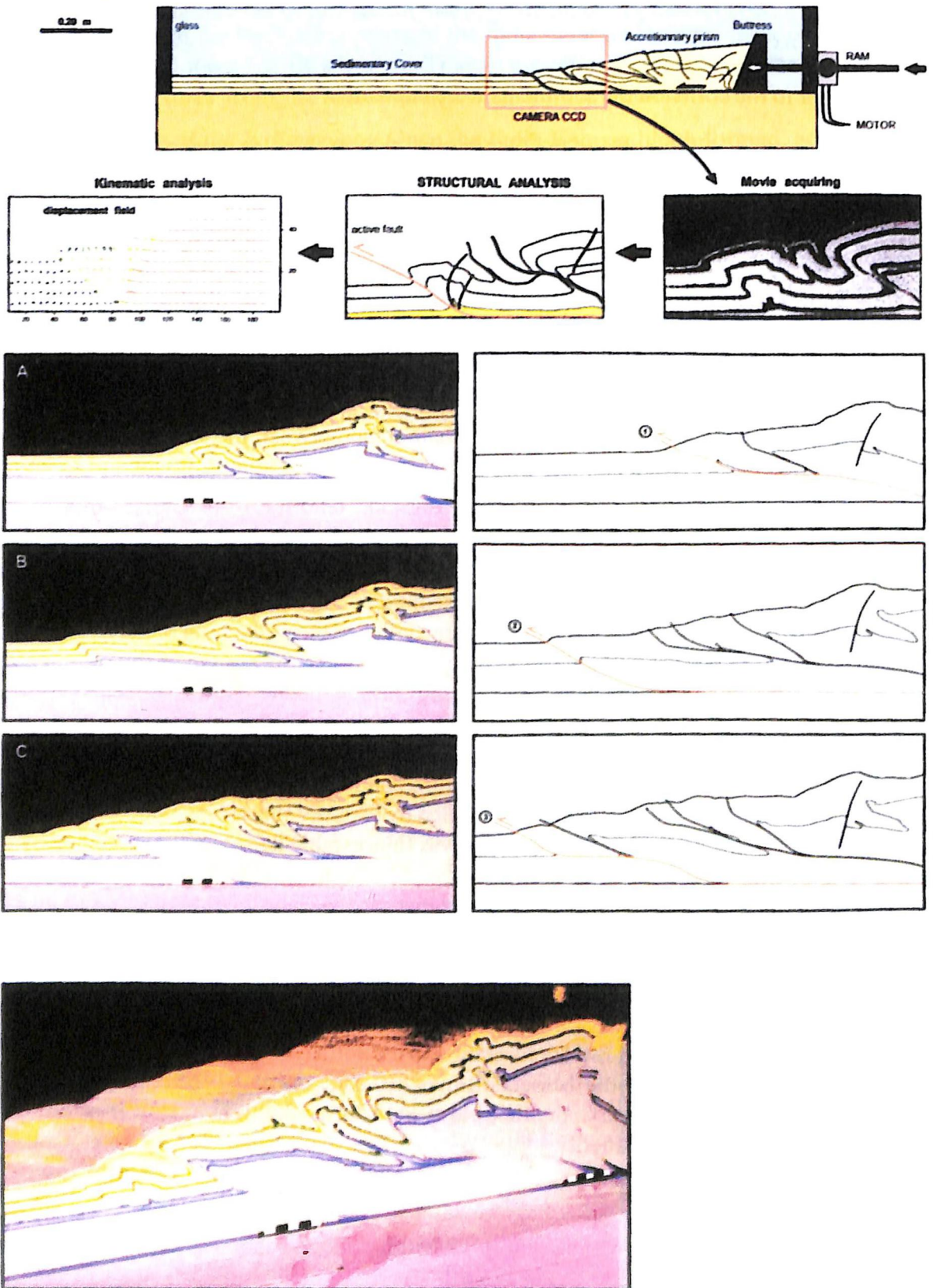
(Frame 3) Figure 11 : Analogue modelling of frontal thrusts.
