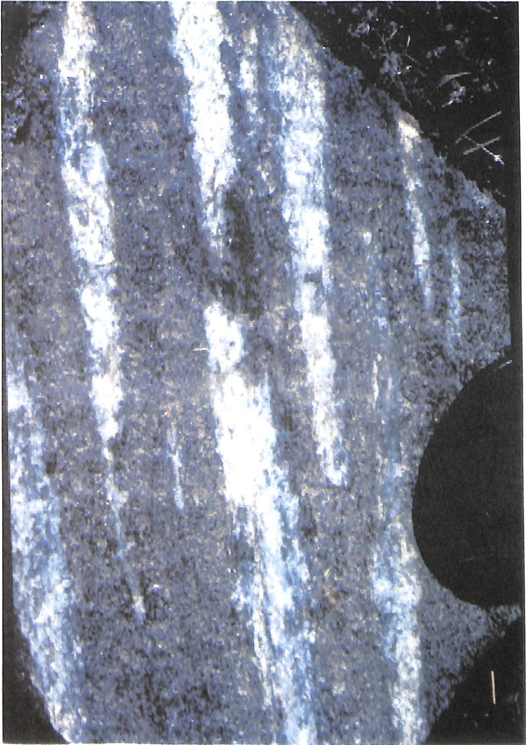
Figure 6: Sillimanite fibers in the Tibetan slab indicative of the stretching towards the transport direction.
